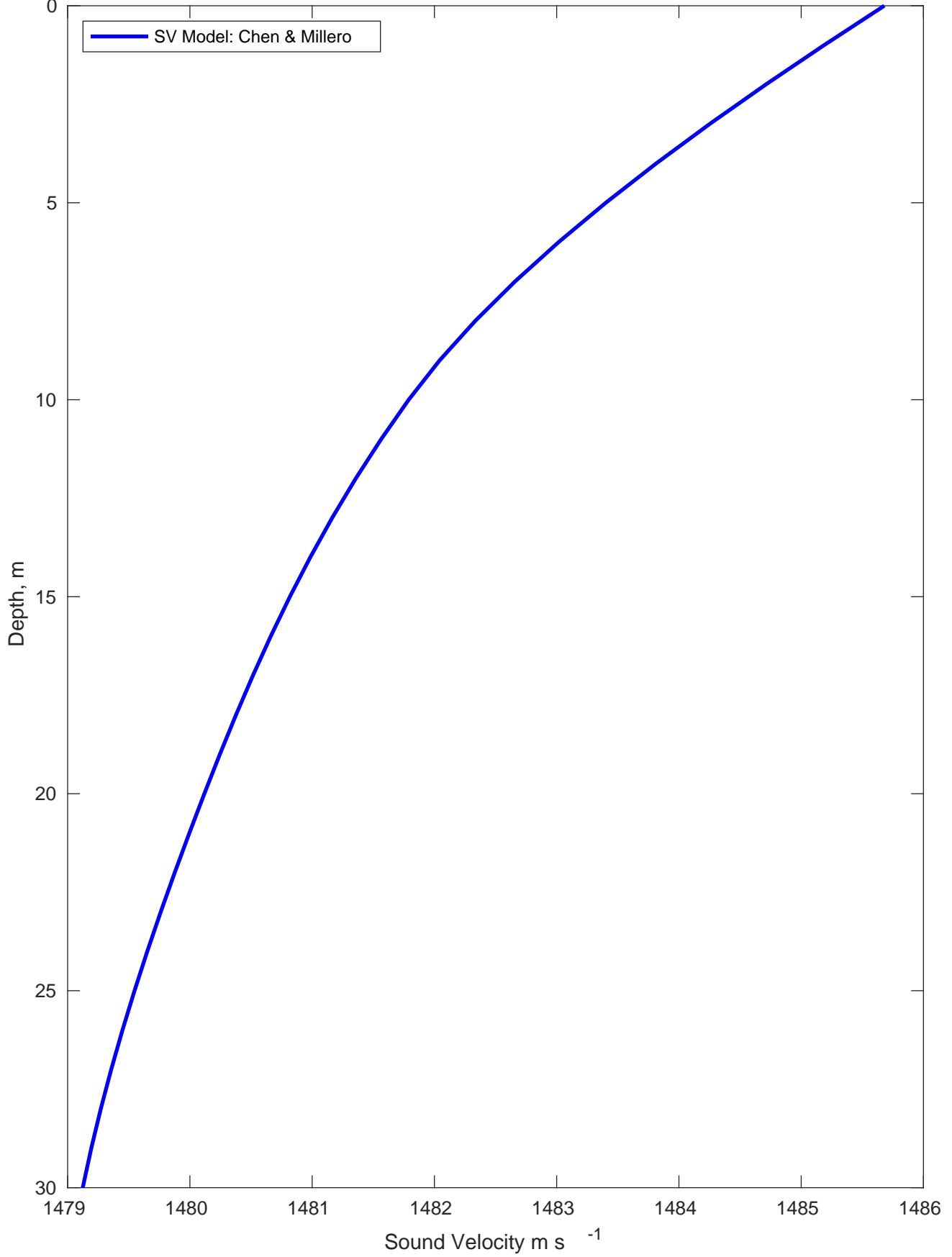
Sound Velocity Profile for Vineyard Mid Atlantic OCS-A 0544 on 02-May-2024 00:00:00
